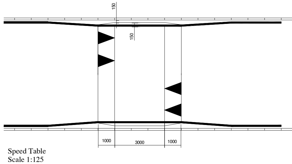
Figure 20.3 - Tapered Edge Speed Table and Road Hump
