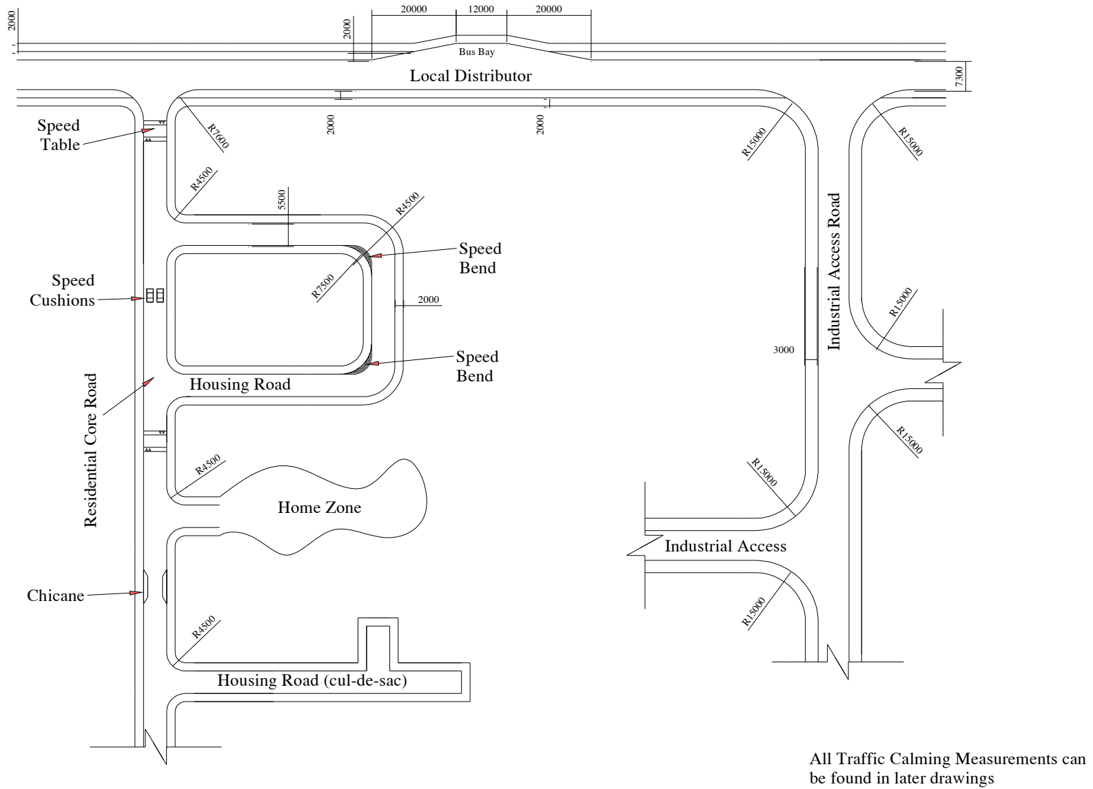
Figure 8.1: Sample Layout of General Access Roads and Culs-de-sac
