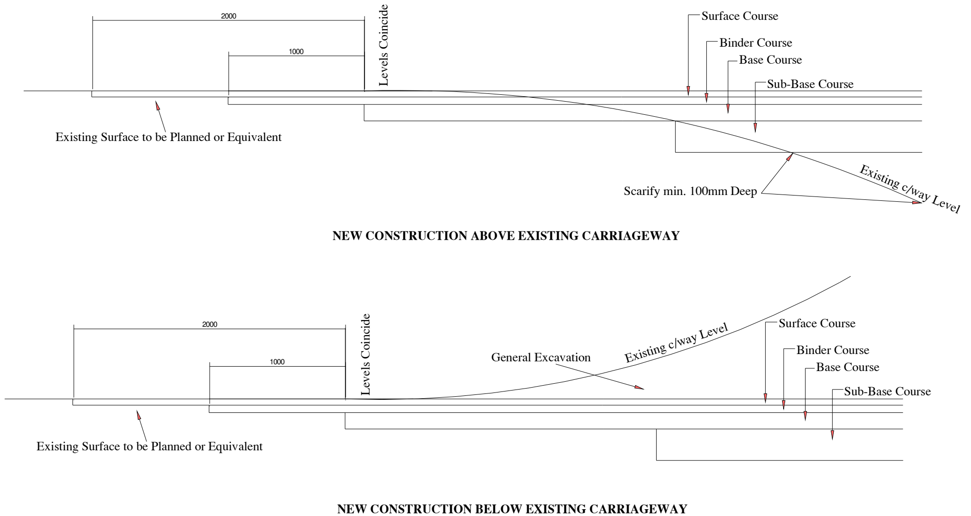
Figure 30.2 - Longitudinal Tie in Details
