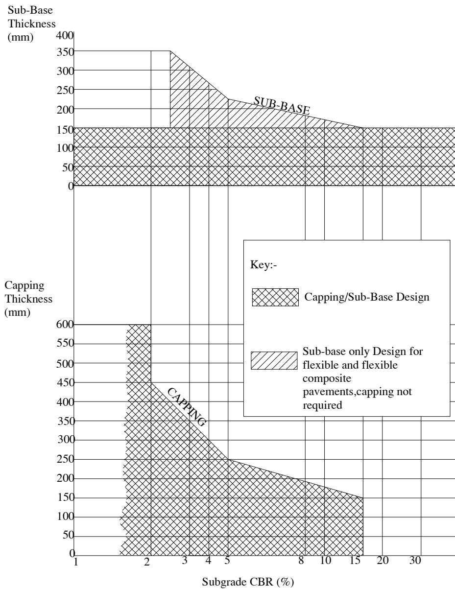
Figure 30.1: Capping and Sub-base A
