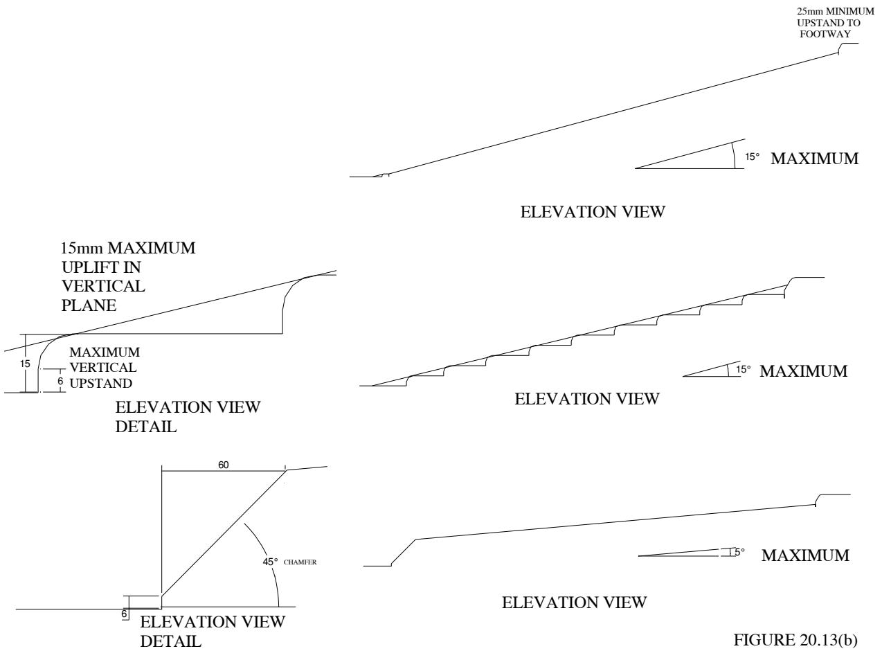
FIGURE 20.13 - SPEED BEND
