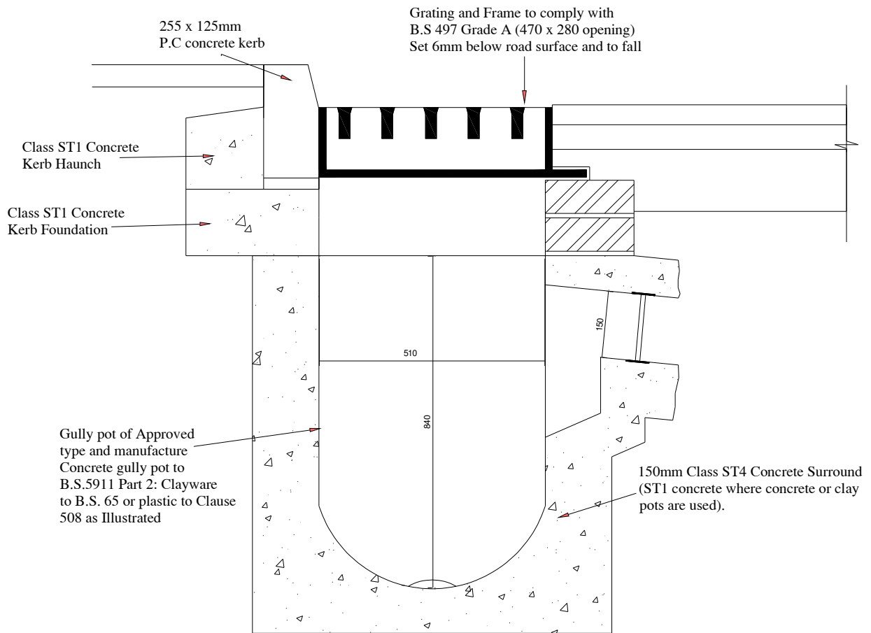
Figure 31.1 - Typical Road Gully
