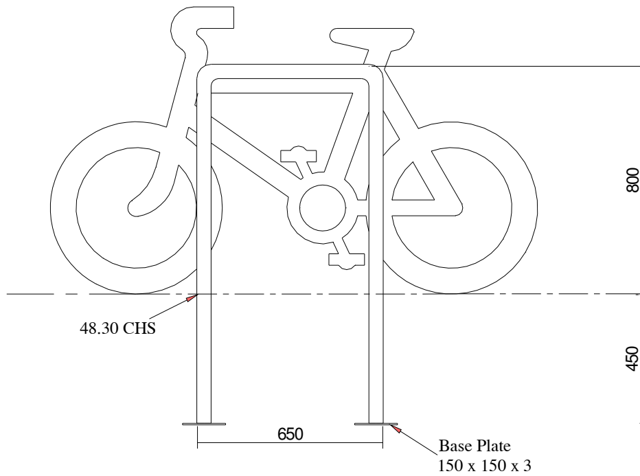
Figure 22.1 - 'Sheffield' Cycle Racks
