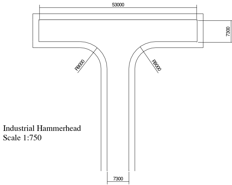
Figure 19.2: Industrial and Residential Hammerhead A
